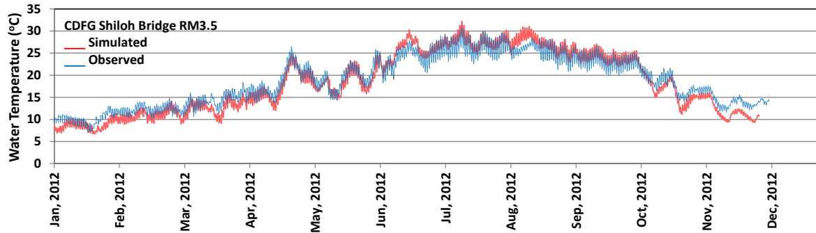
Figure 5.2-2. Model validation using calendar year 2012.
