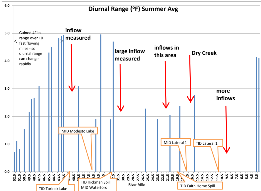
Figure 5.4-5. Summer average diurnal range (2011) at actual river location – annotated with return flow locations.
