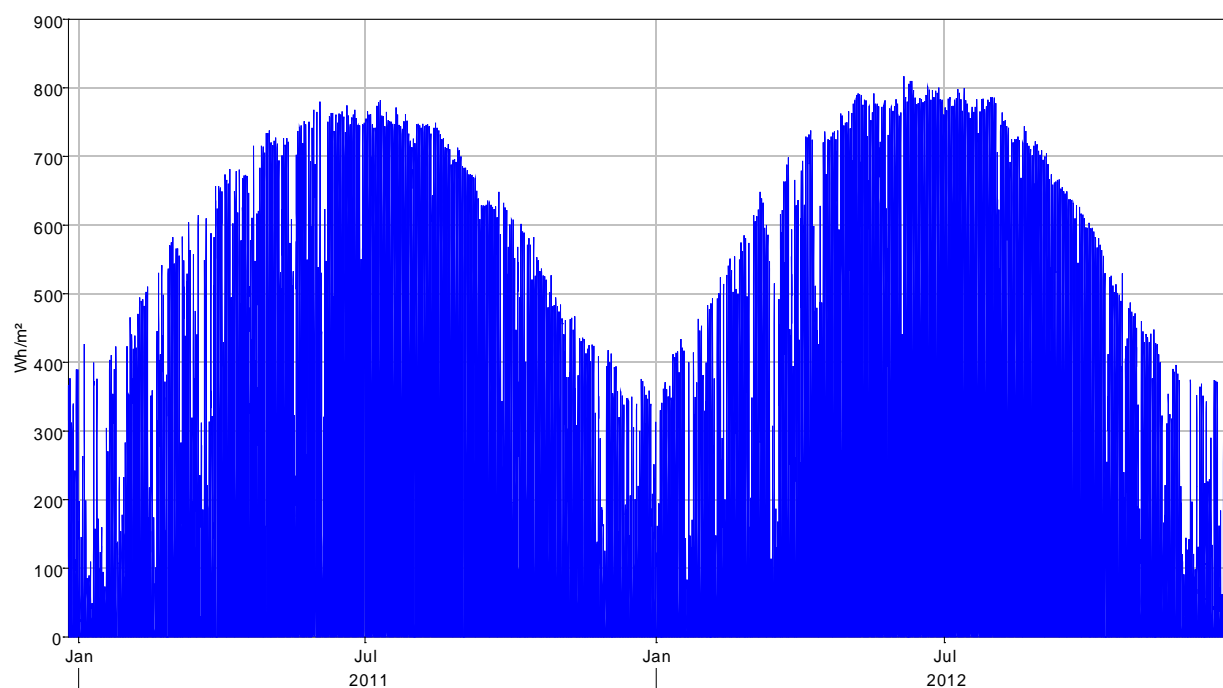
Figure 4.3-7. Denair short wave radiation used in HEC-RAS.
