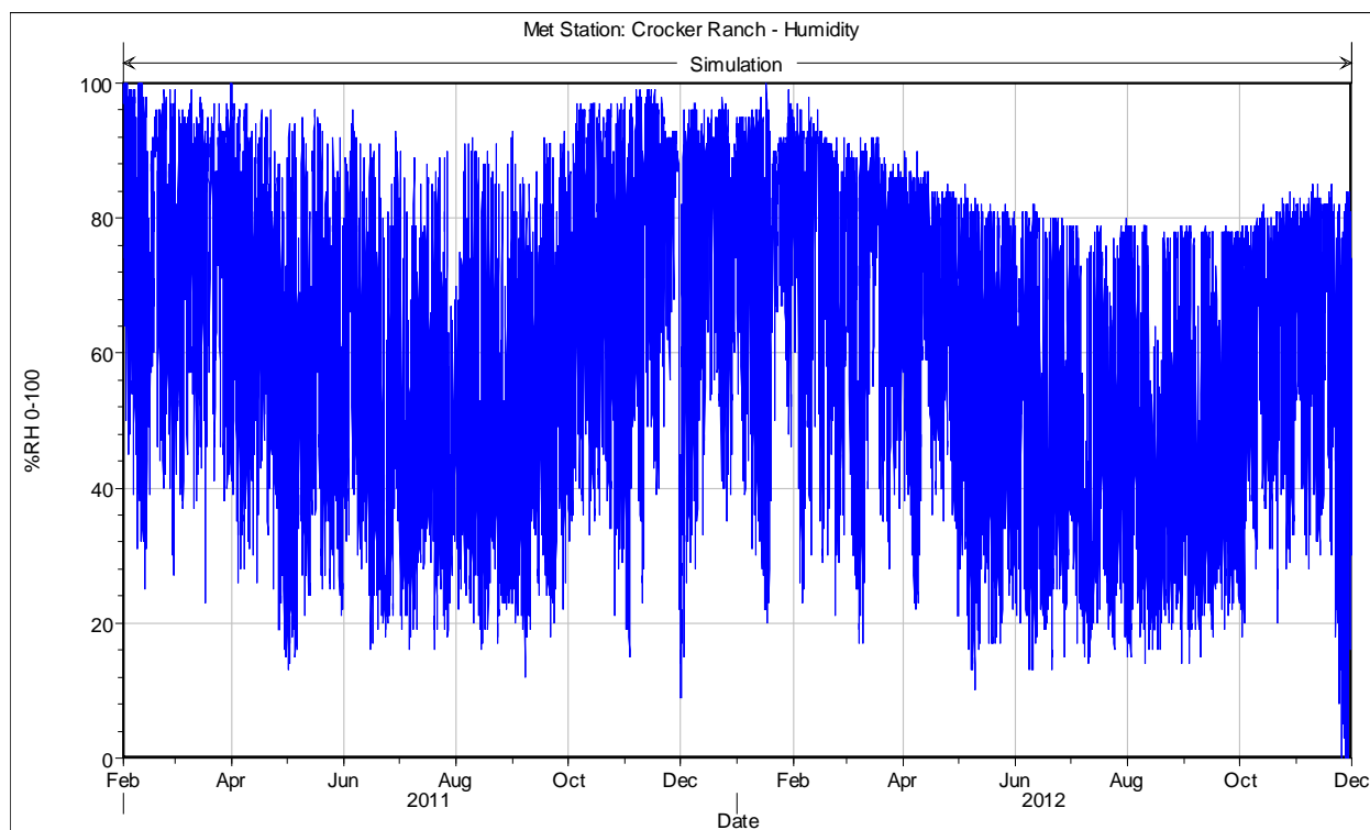
Figure 4.2-4. Crocker Ranch relative humidity for 2011-2012.
