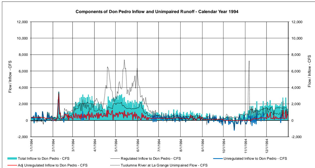
Figure 2.2-24. Calendar Year 1994.
