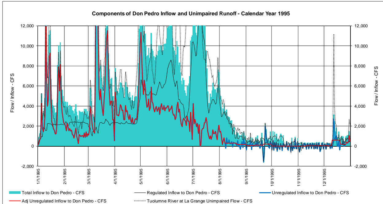
Figure 2.2-25. Calendar Year 1995.
