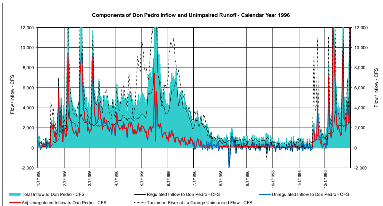
Figure 2.2-26. Calendar Year 1996.
