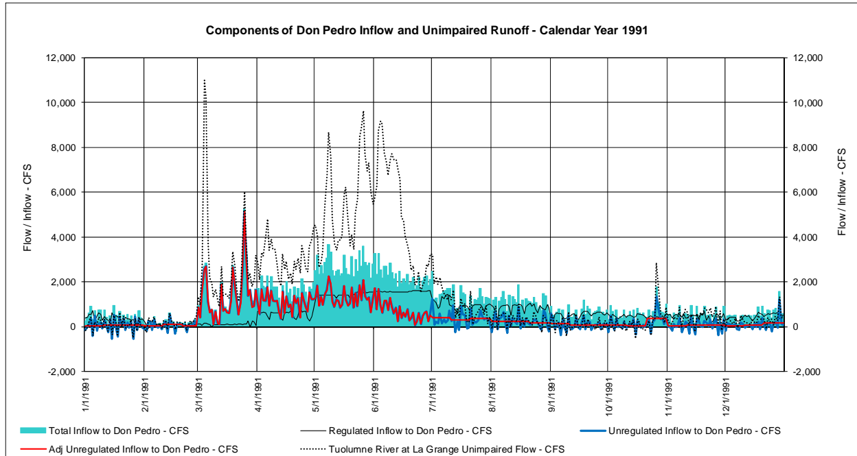
Figure 2.2-21. Calendar Year 1991.
