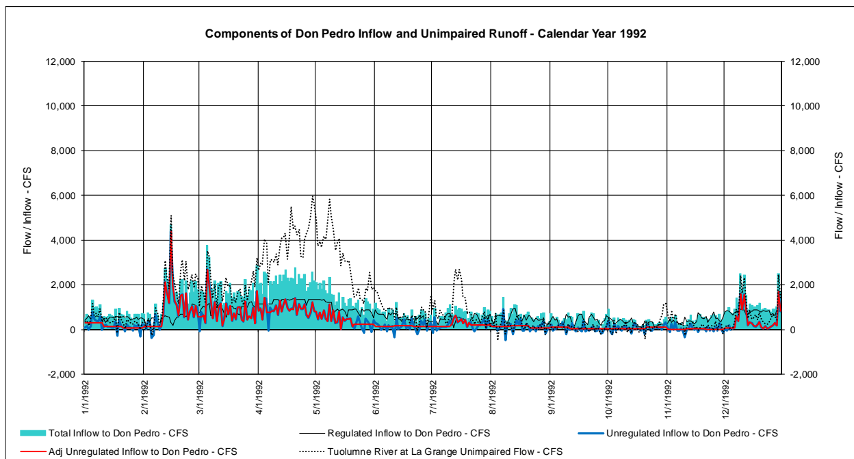
Figure 2.2-22. Calendar Year 1992.
