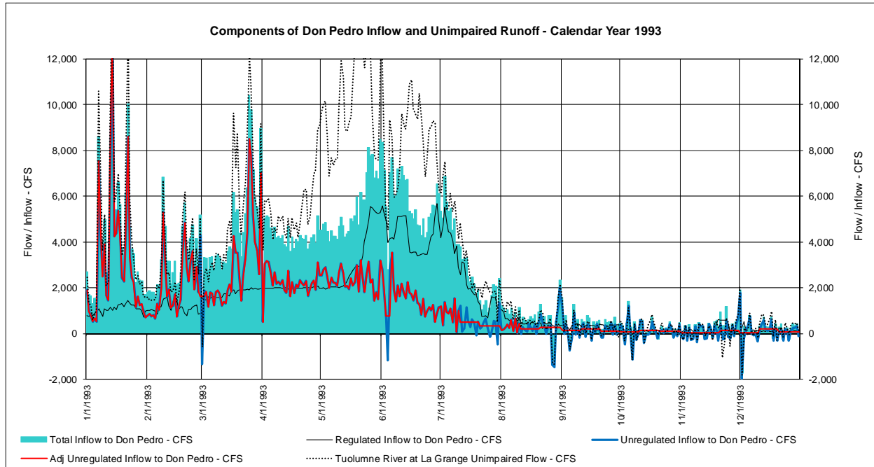
Figure 2.2-23. Calendar Year 1993.
